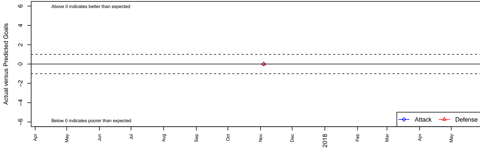
San Juan SC USSDA B05 Dots are actual minus expected GF (blue circles) and GA (red triangles). Blue line is smoothed change in attack strength. Red is smoothed change in defense strength.
